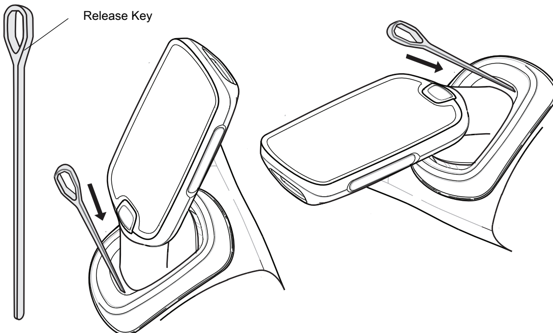
Figure 82 Manual Release of the PS20 from a Three Slot Cradle
