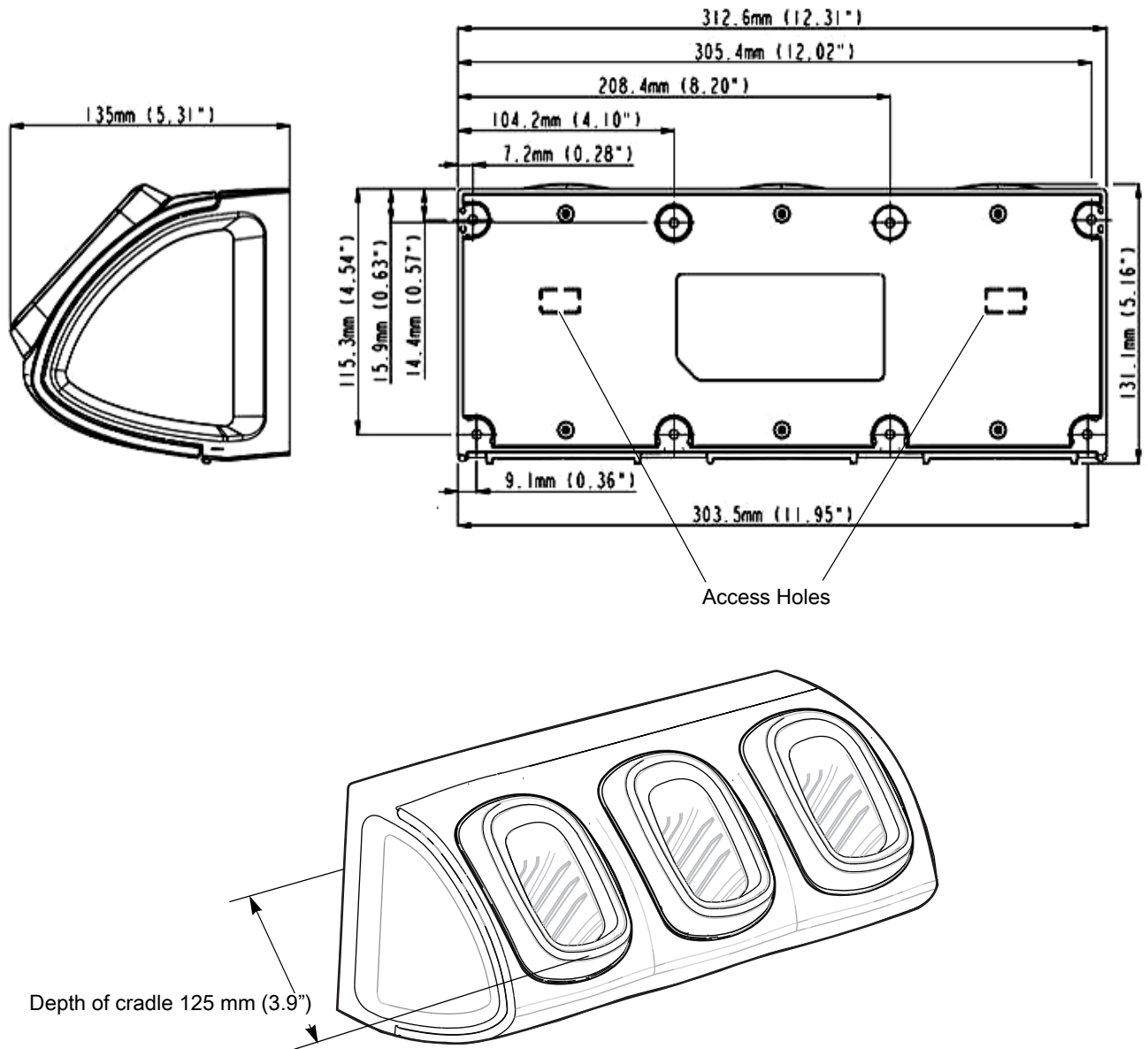
Figure 72 Three Slot Cradle - Mounting Template and Overall Depth
