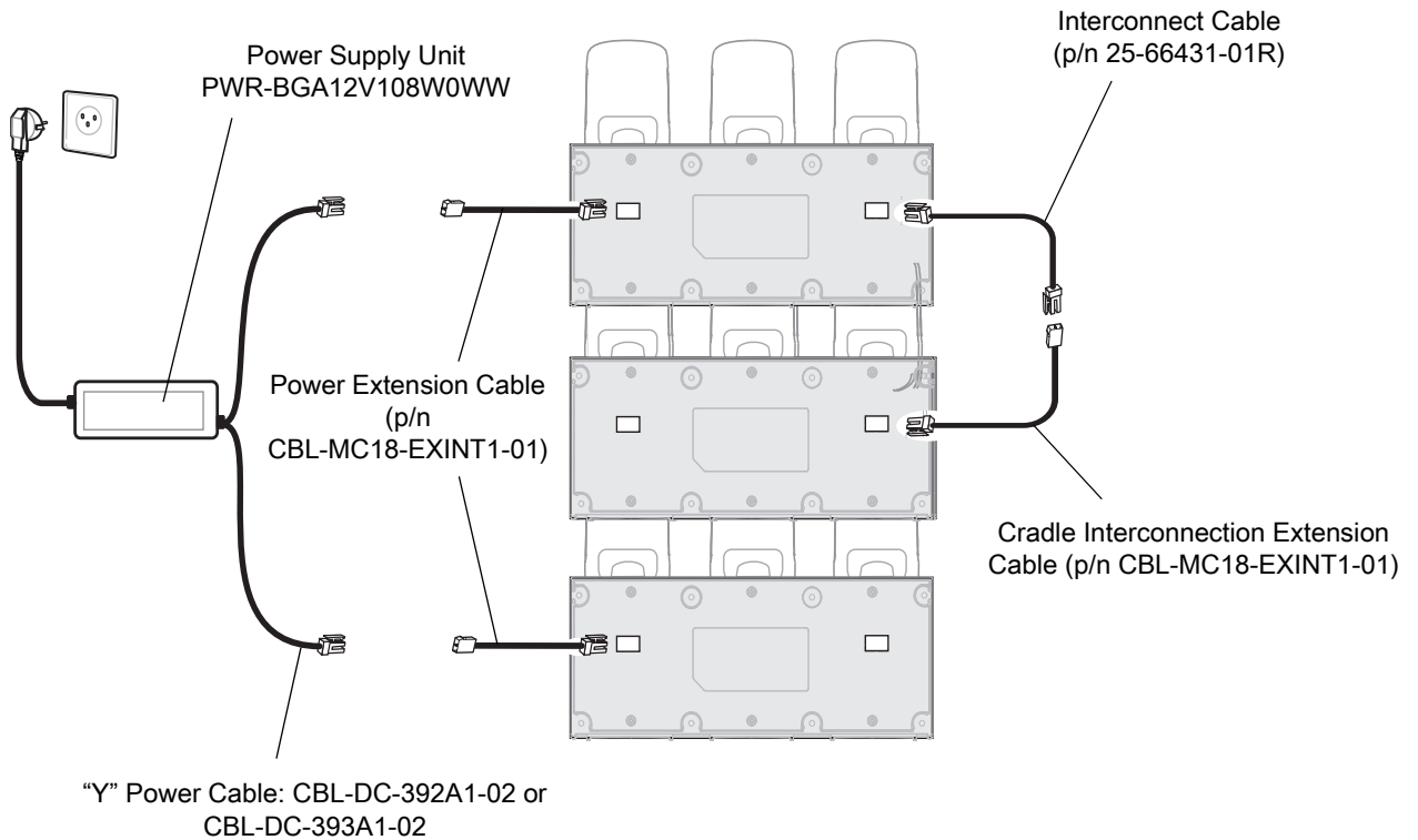
Figure 71 Fast Charging Mode Cable Connections
