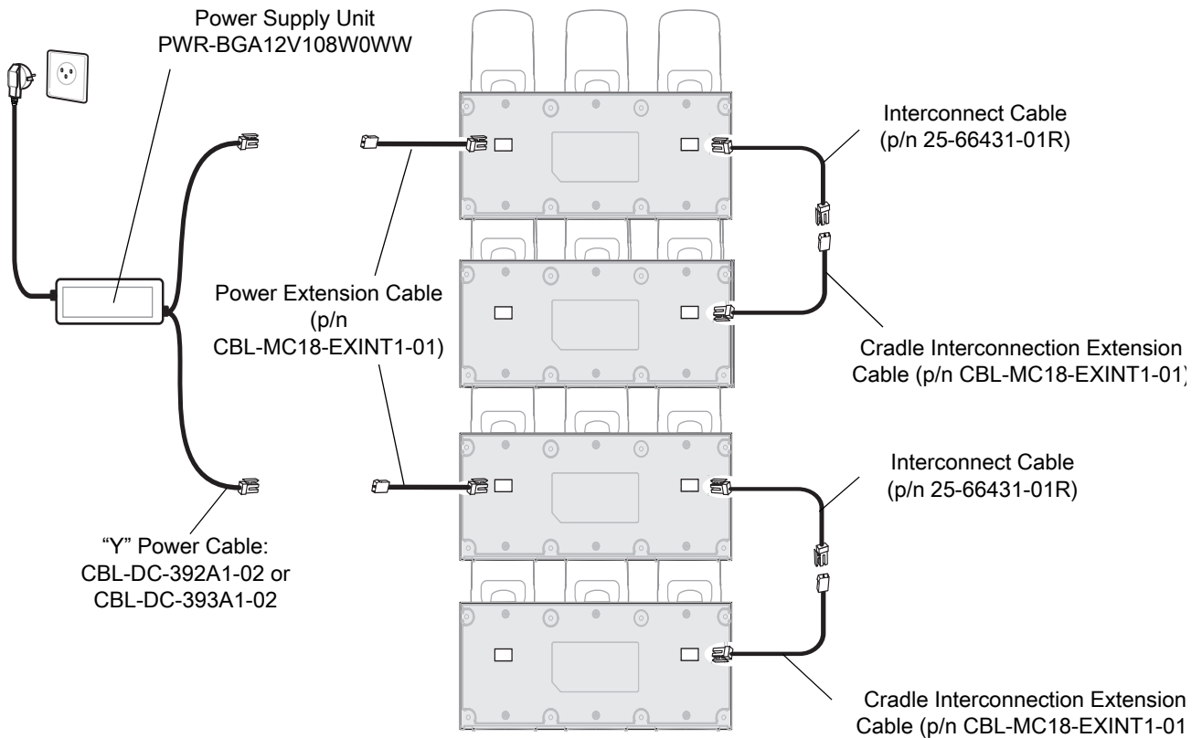
Figure 70 Standard Charging Mode - Cable Connections
