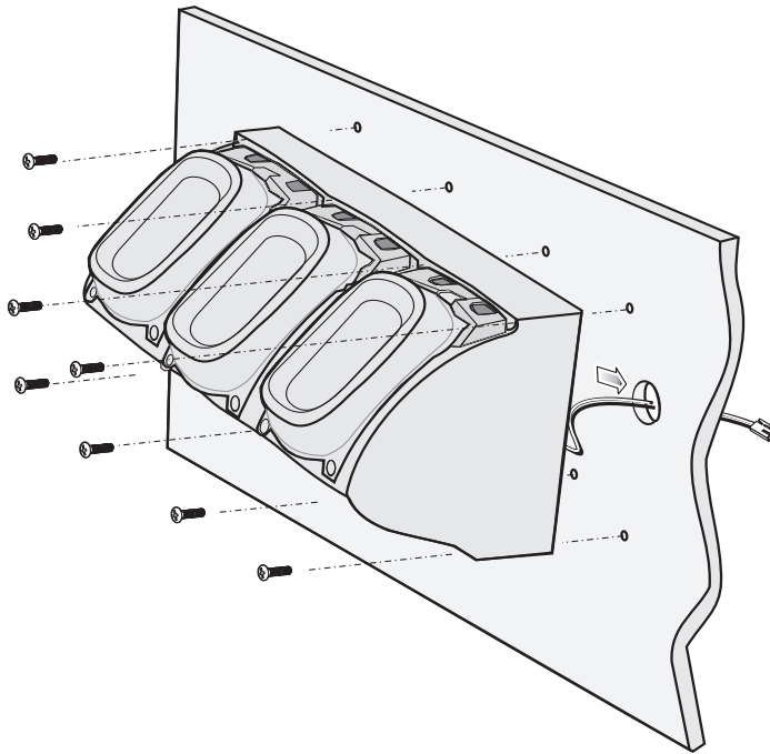
Figure 78 Three Slot Cradle - Fastening the Cradle to a Wall
