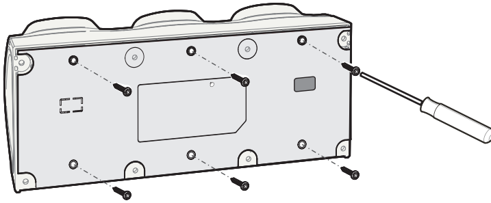
Figure 76 Three Slot Cradle - Securing the Back Cover
