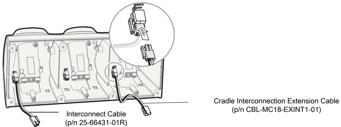
Figure 73 Three Slot Cradle - Cable Connections
