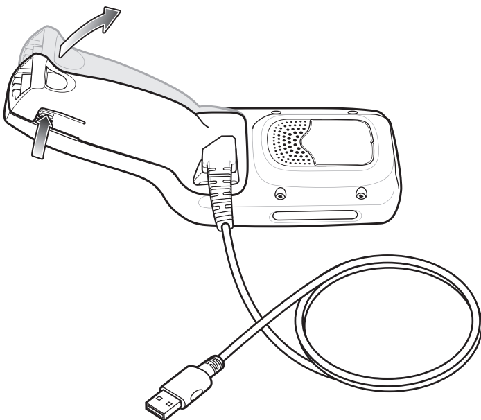
Figure 85 Remove USB Cable Battery Cover
