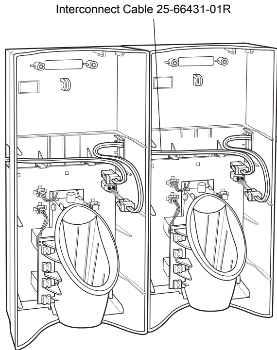
Figure 60 Daisy-Chaining Cradles
