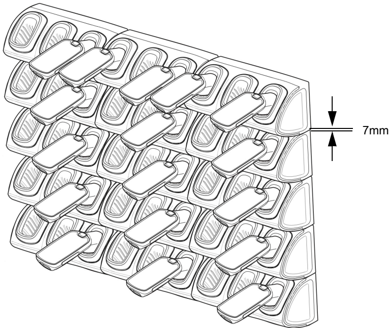
Figure 68 Installation in Super High Density Configuration
