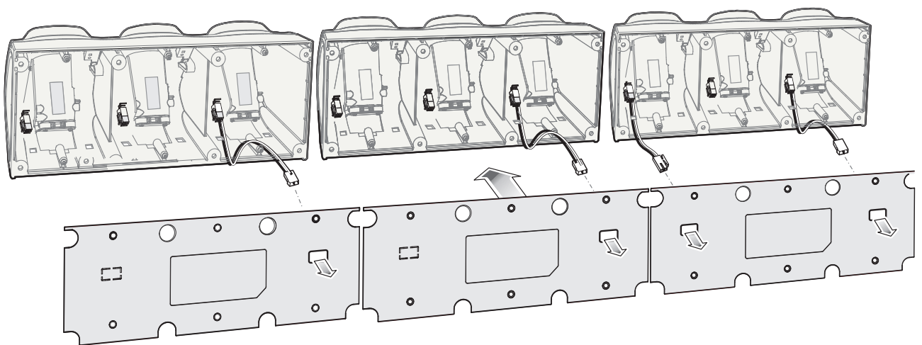
Figure 75 Three Slot Cradle - Back Cover Cable Routes
