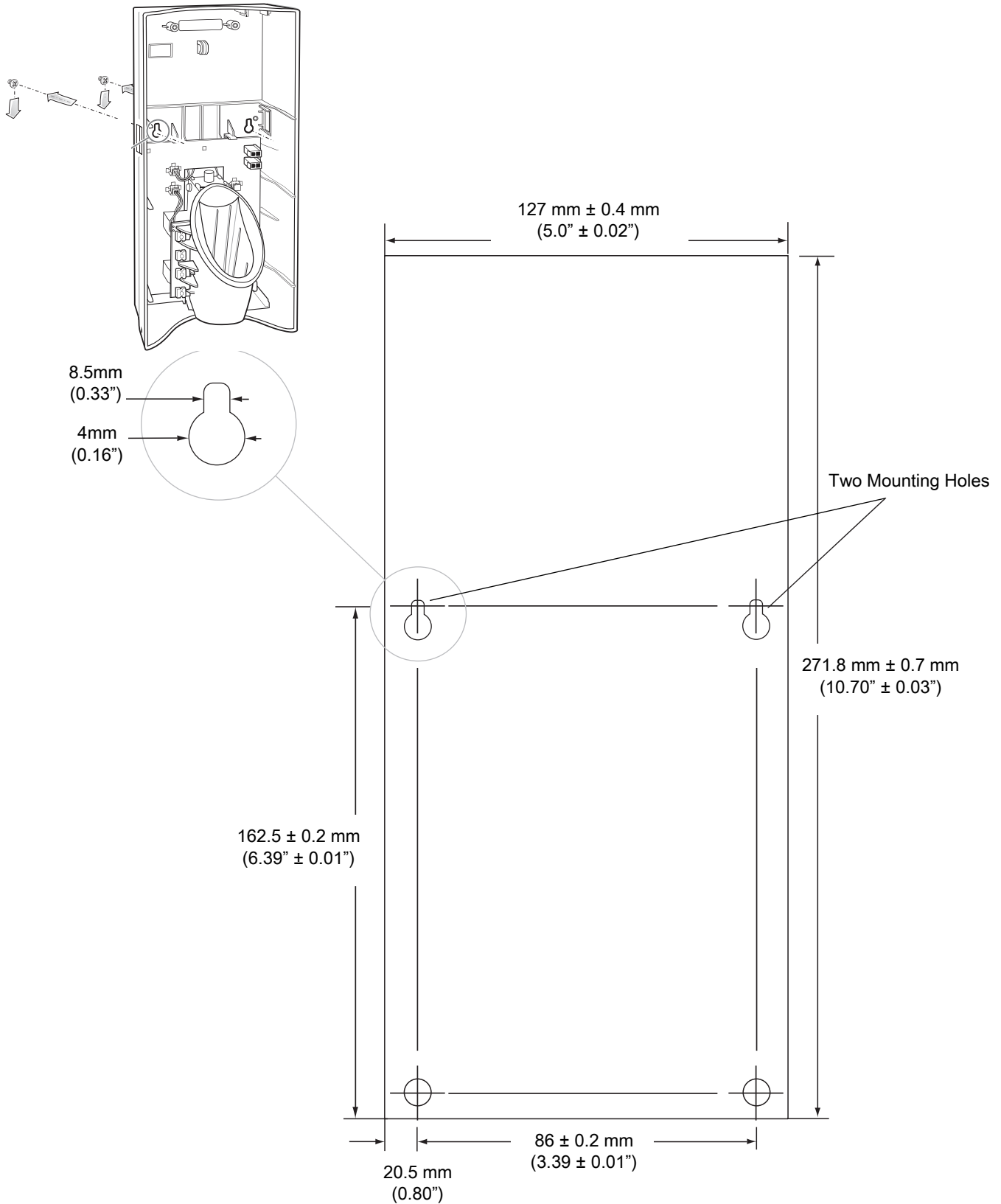
Figure 57 Hanging the Cradle on a Wall - Mounting Template
