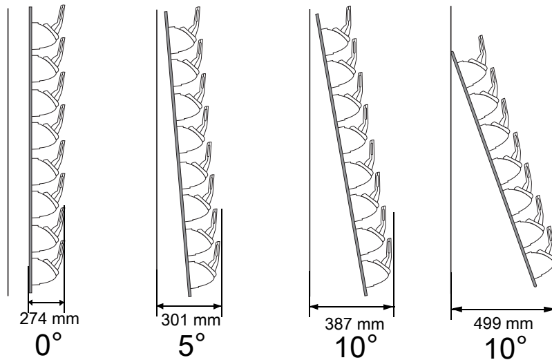
Figure 67 Dispenser Wall Angles
