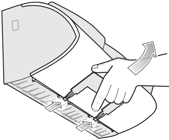
Figure 77 Three Slot Cradle - Removing Front Cover
