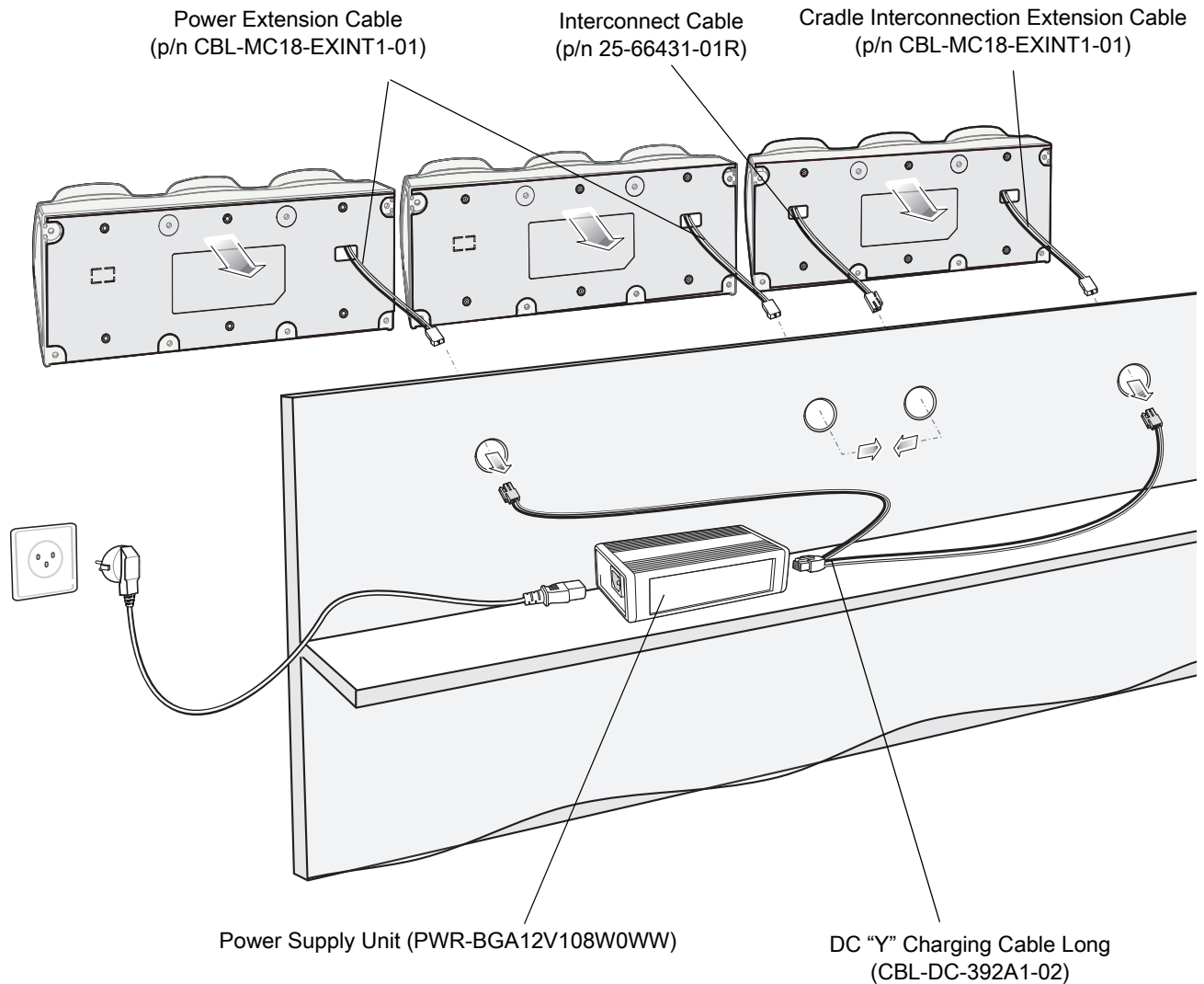
Figure 80 Three Slot Cradle - Connection to Power Supply Unit
