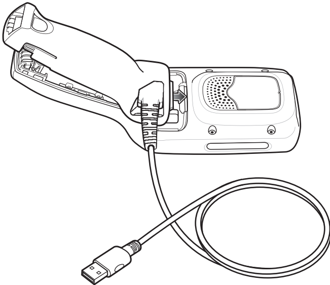
Figure 83 Install USB Cable Battery Cover - Top
