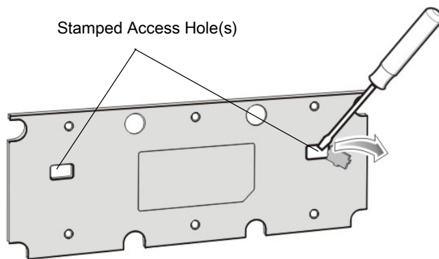
Figure 74 Three Slot Cradle - Stamped Access Hole(s)
