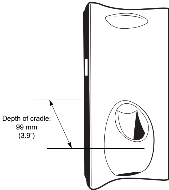
Figure 58 Overall Depth of Cradle
