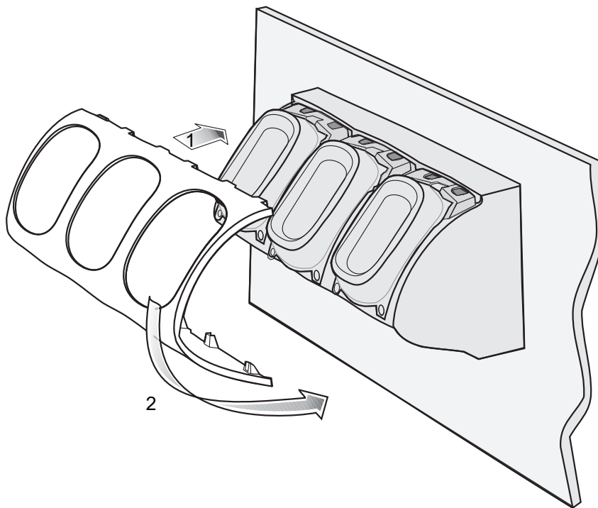
Figure 79 Three Slot Cradle - Connecting the Front Cover
