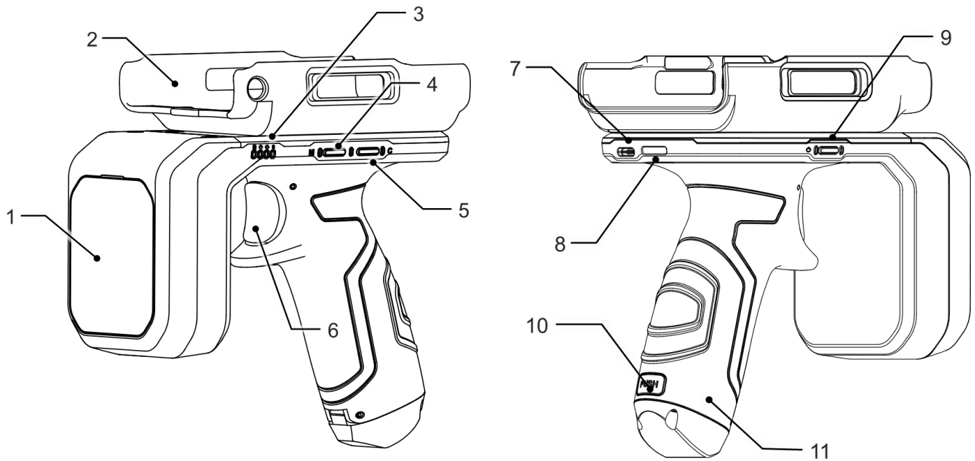
Figure 1 RF851 Views
