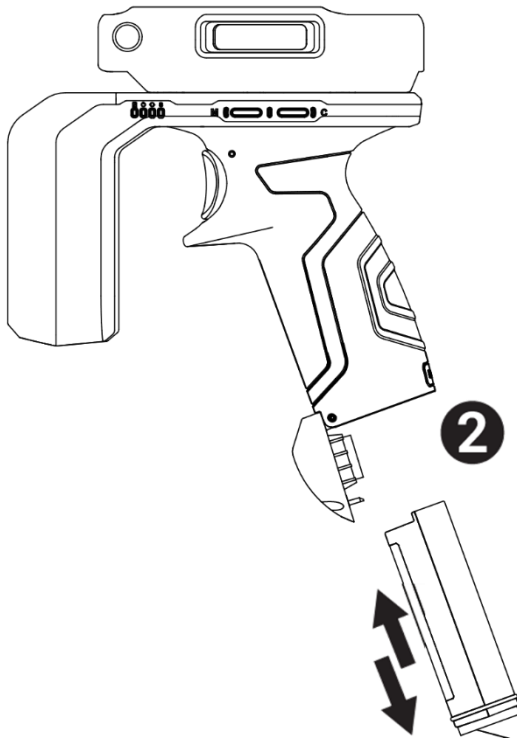
Figure 7 Replace battery
