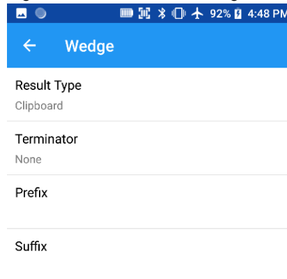
Figure 33 RFID Control - Wedge
