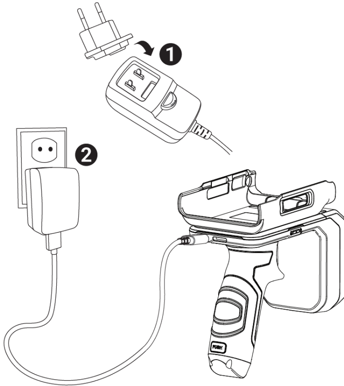
Figure 2 Charge RF851
