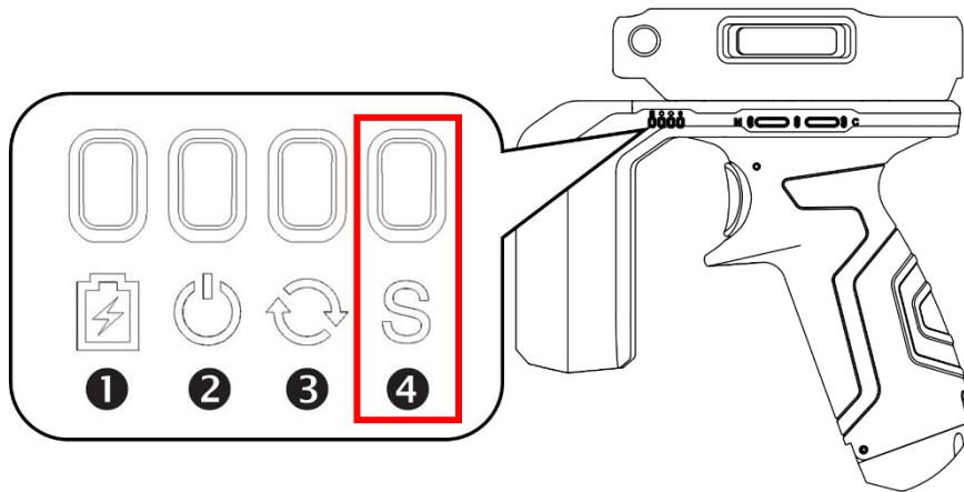
Figure 36 RF851 Trigger-Mode LED
