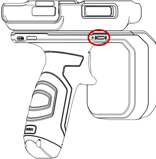
Figure 5 RF851 Power button
