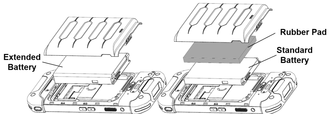
Figure 10 Battery cover and rubber pad
